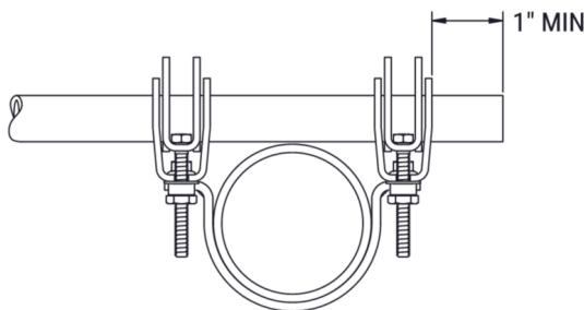
FIG. AF735 cULus & FM Approved Brace Members
